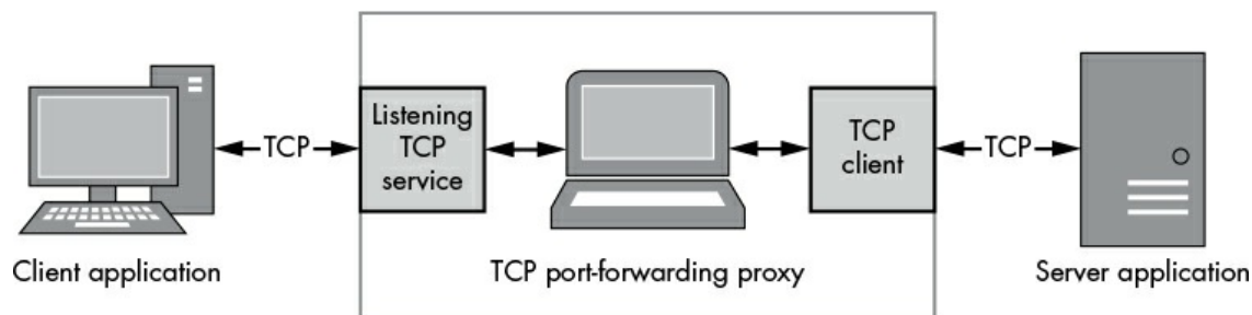
Figure 2-8: Overview of a TCP port-forwarding proxy
