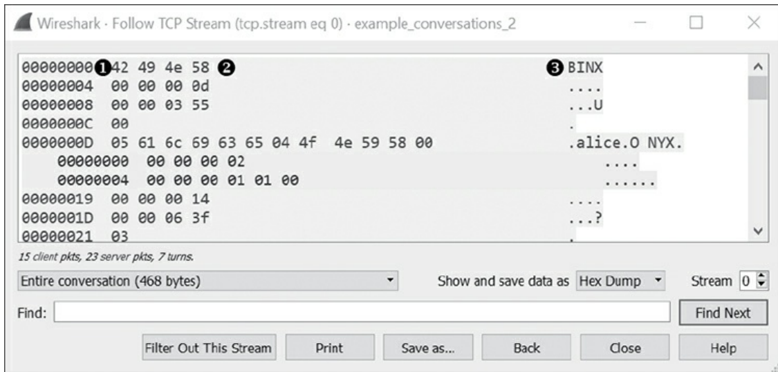
Figure 5-7: The Hex Dump view of the stream
