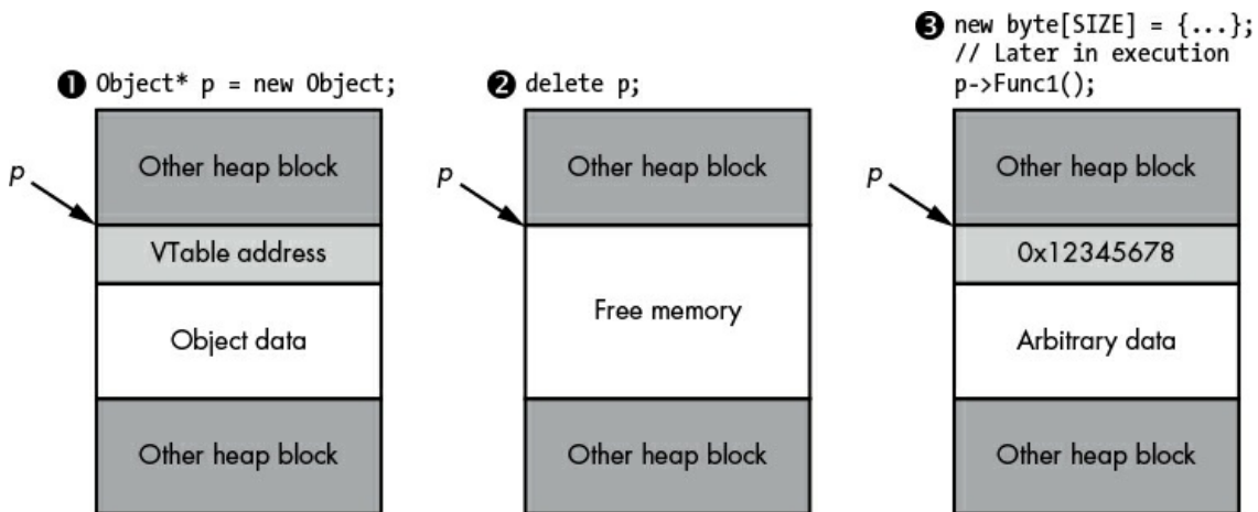
Figure 10-5: An example of a use-after-free vulnerability
